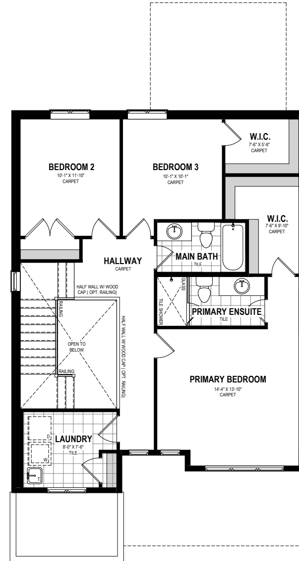
SECOND FLOOR
